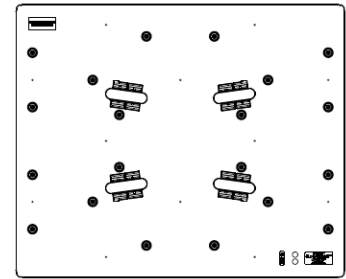
Frictional Element Configuration (20)
